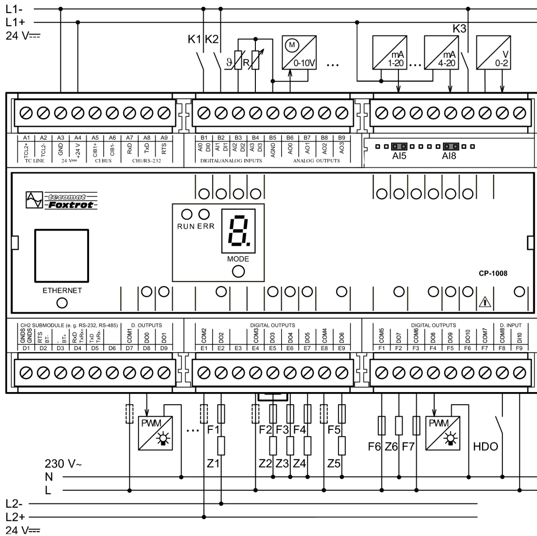
Fig. 4.1 Example connection of binary and analog inputs/outputs of basic module CP-1008
