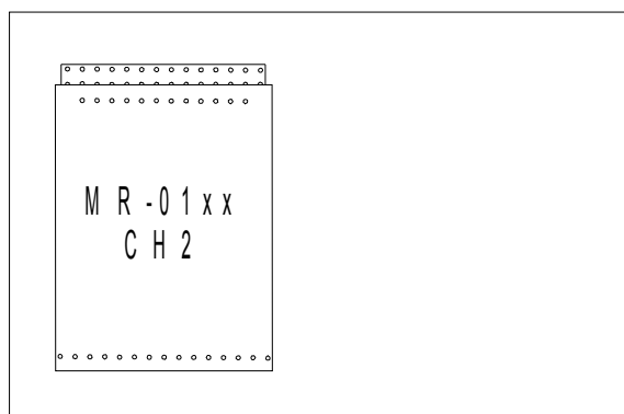
Fig.7.1 Placement of a plug-in submodule with serial interface onto the middle board of the basic module CP-1008
