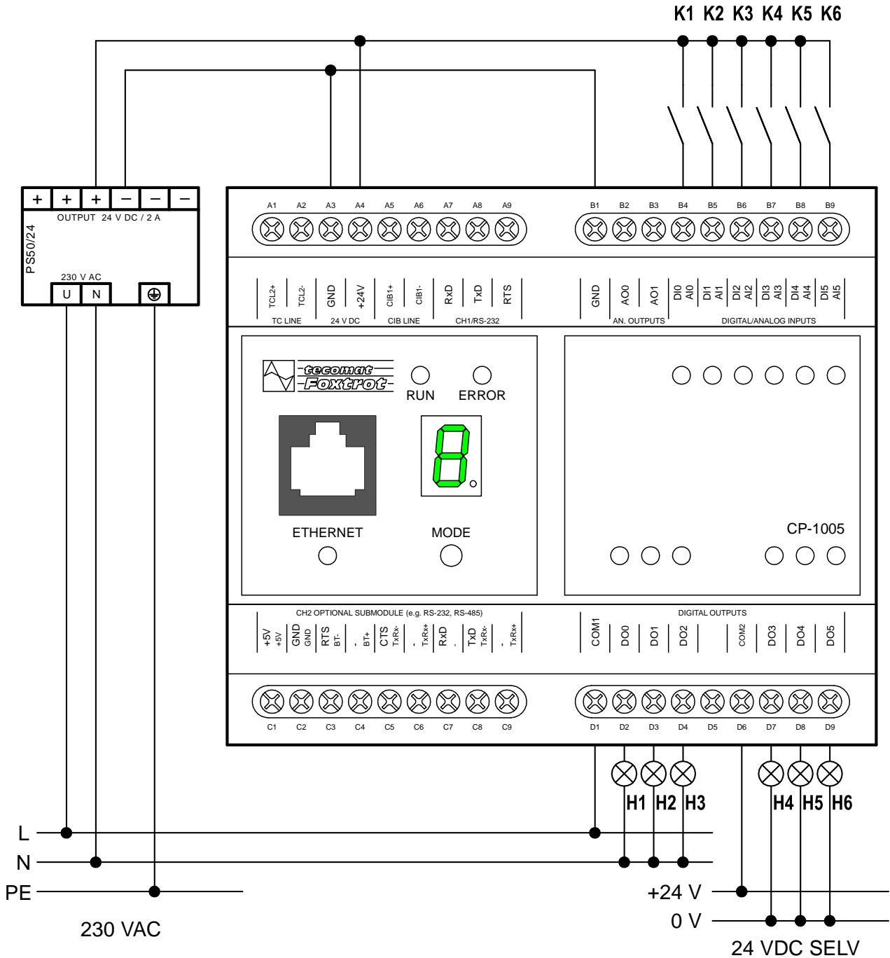
Fig. 4.1 Elementary connection of CP-1005 module
