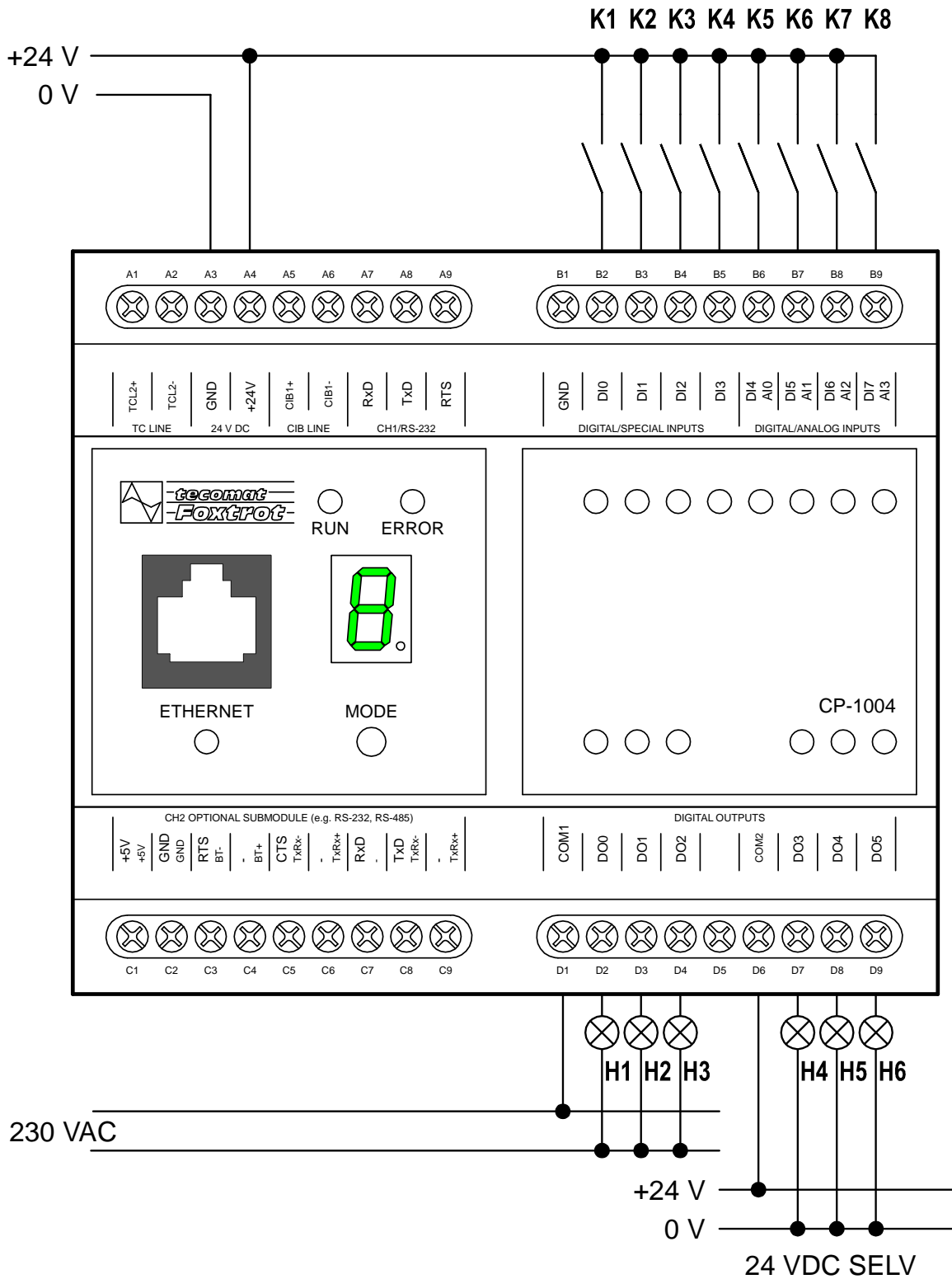
Fig. 5.1 Elementary connection of CP-1004 module
