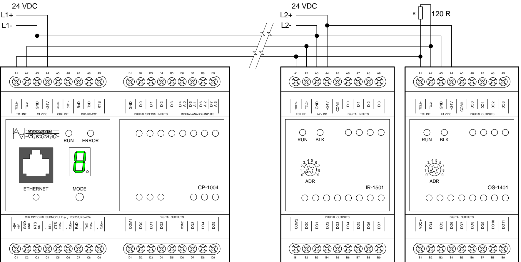
Basic diagram of the TCL2 bus connection without power supply
